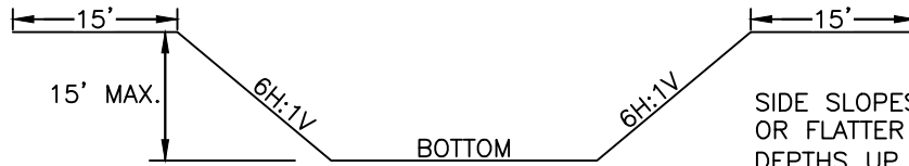
WET POND (15' MAX. VERTICAL DEPTH)
